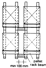
⑦ Device to stop pallet racks from sliding
